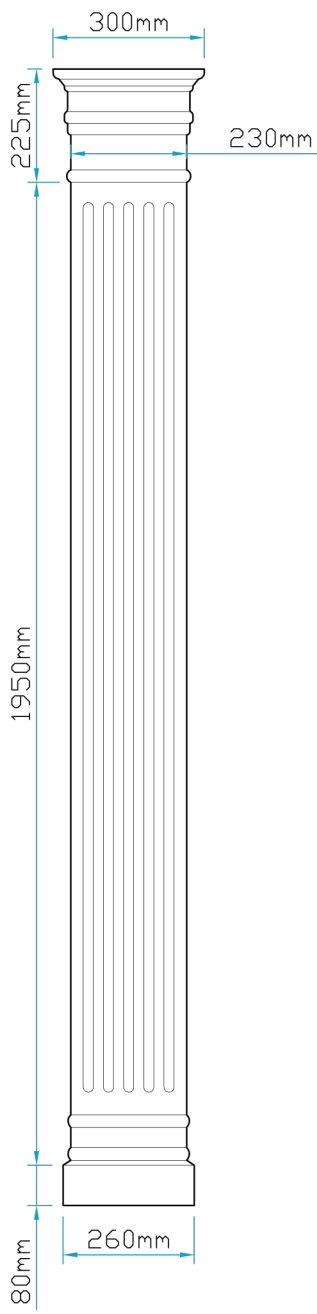
Front Elevation
