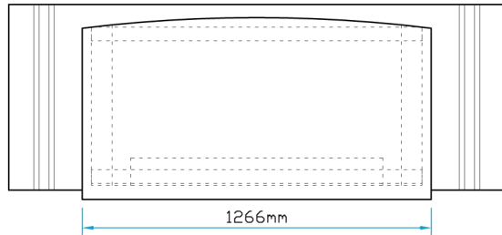
Plan View
