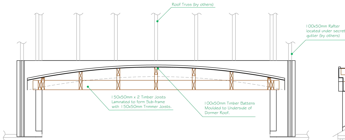
Section B-B
