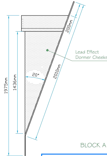
Side Elevation
