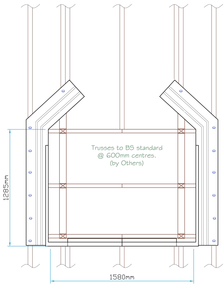
Plan View
