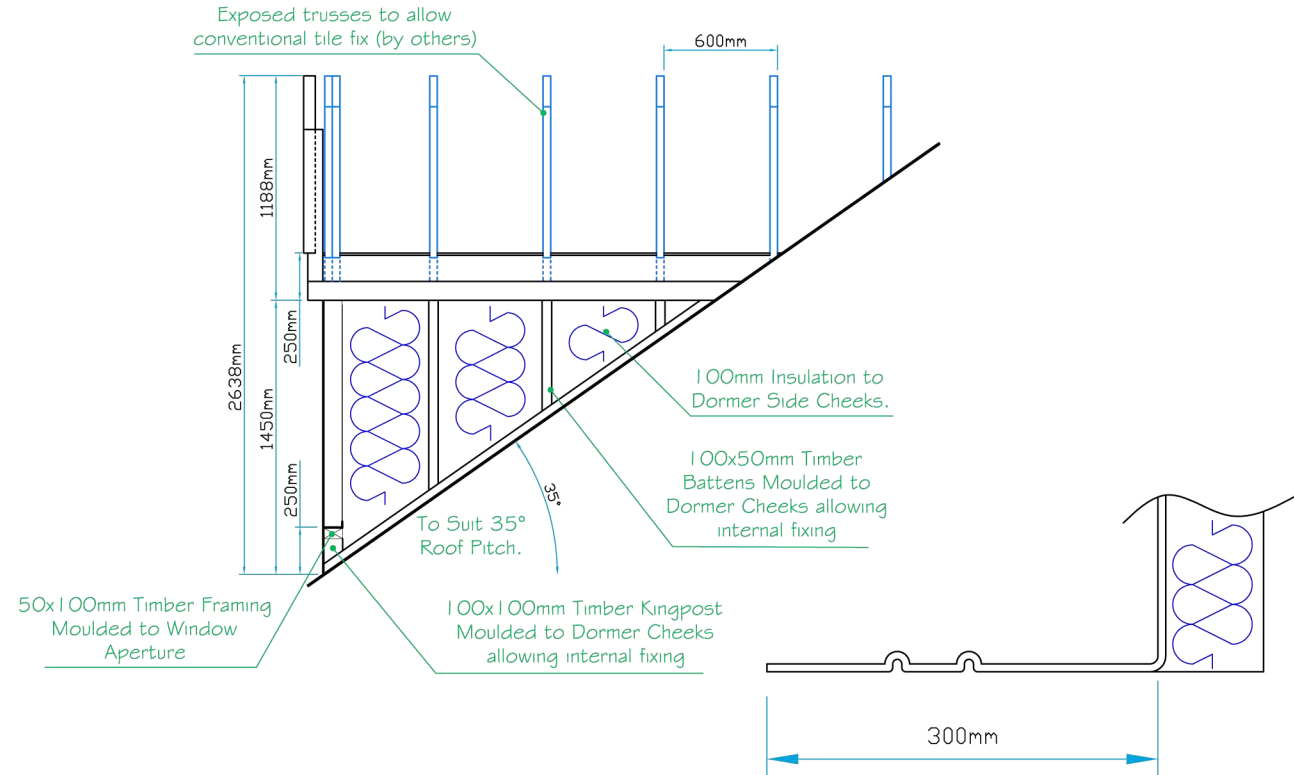
Section B~B
