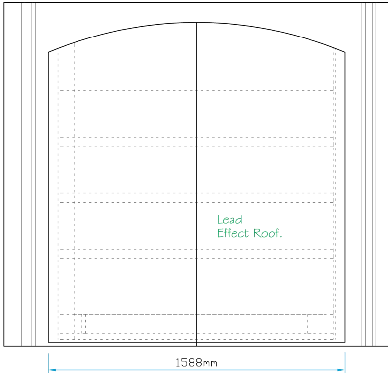
Plan View
