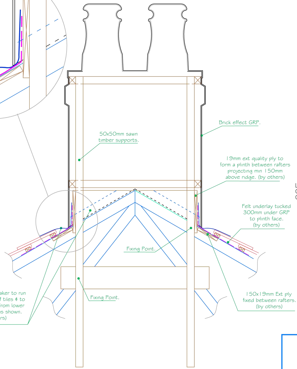
Section A~A
