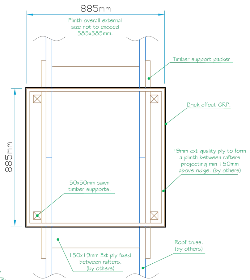
Section B~B
