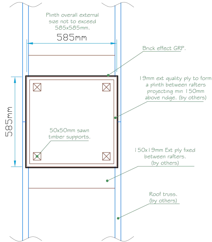
Section B~B
