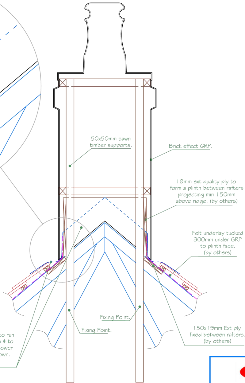
Section A~A
