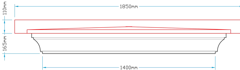
Front Elevation
