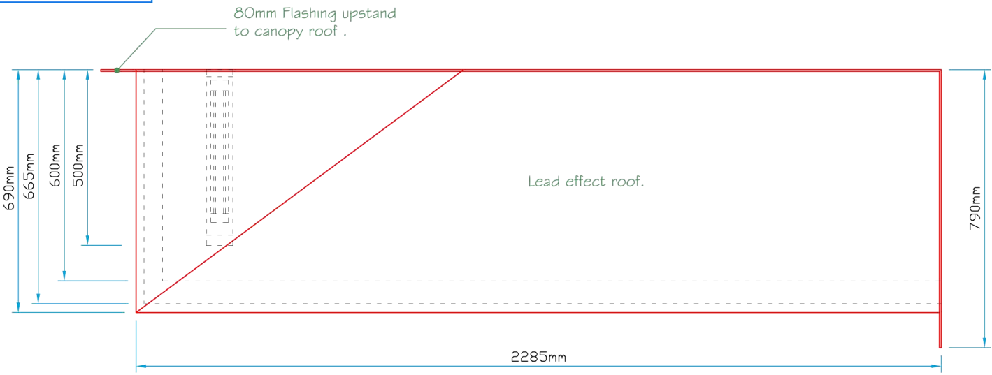
Plan View
