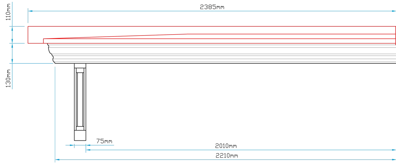
Front Elevation
