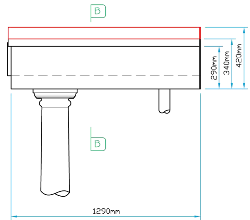
Side Elevation
