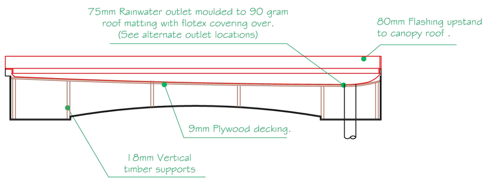
Section B~B
