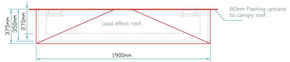
Plan View
