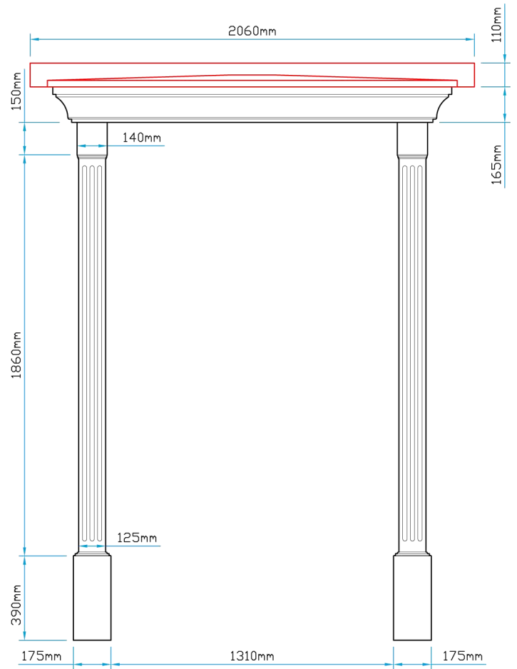
Front Elevation
