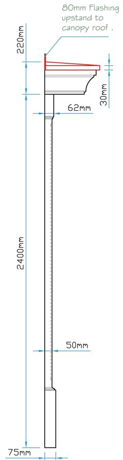
Side Elevation
