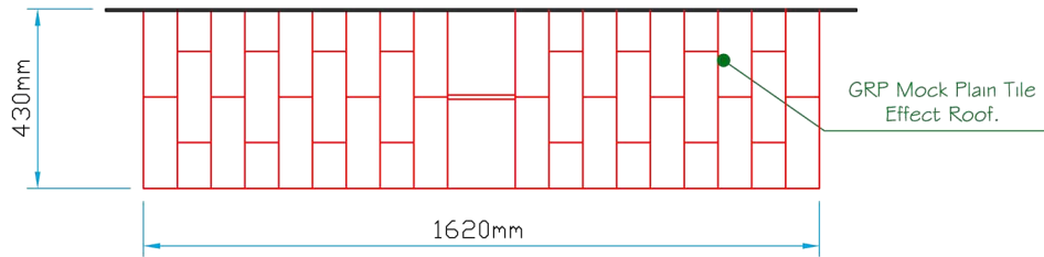
Plan View
