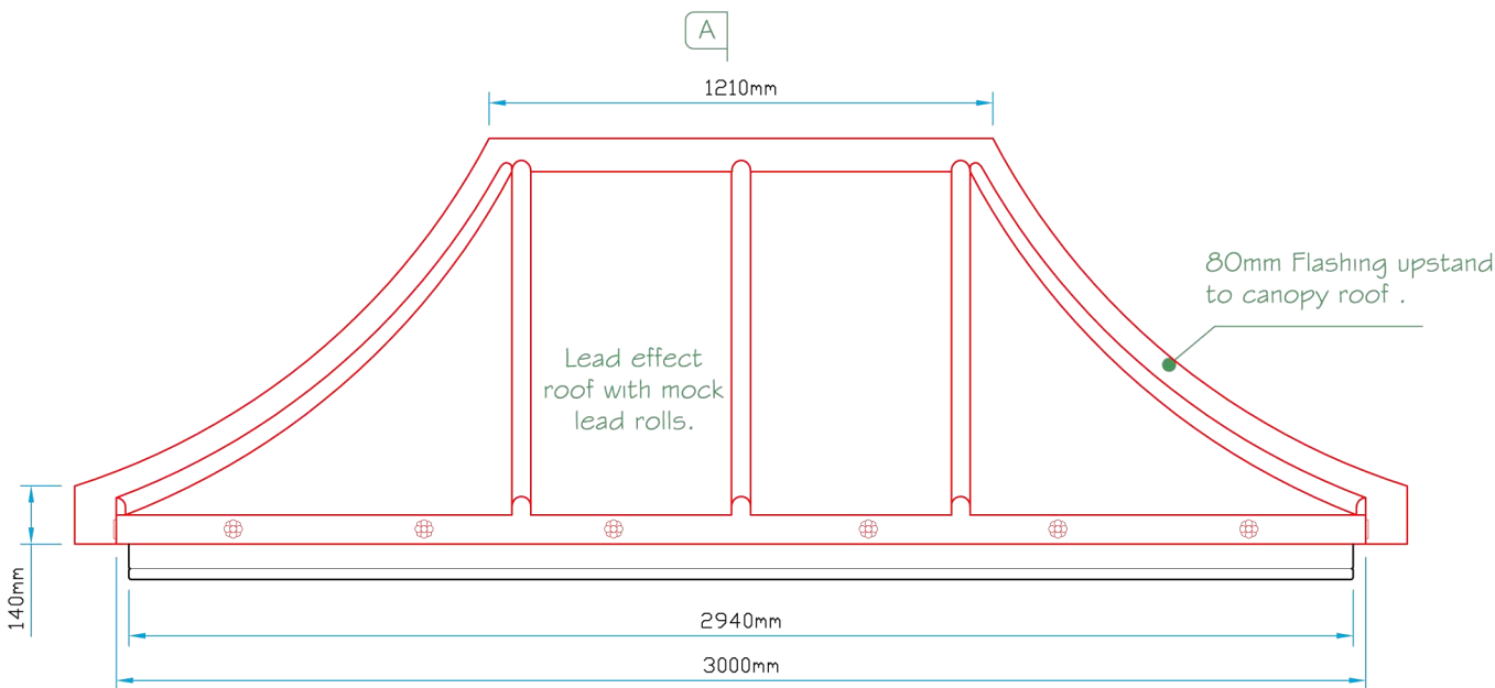
Front Elevation
