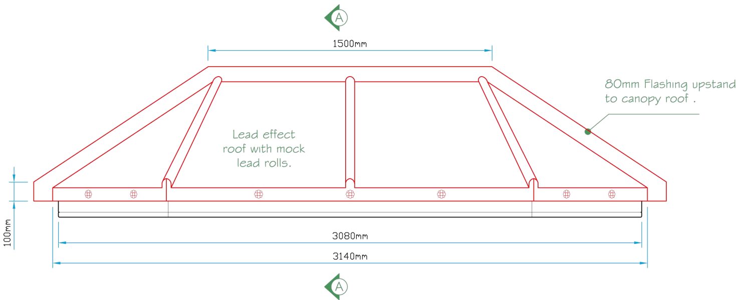
Front Elevation
