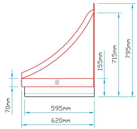
Side Elevation
