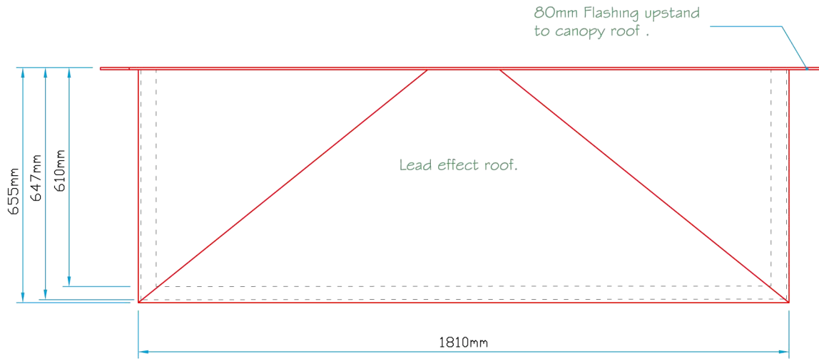
Plan View
