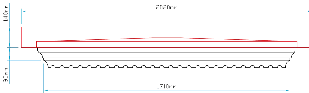
Front Elevation
