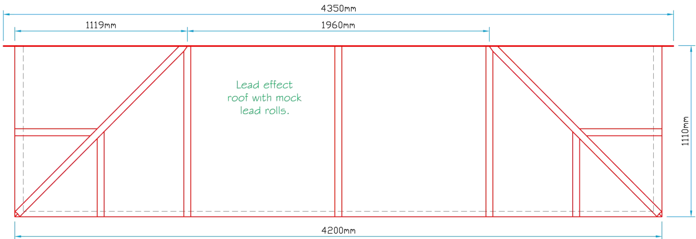
Plan View
